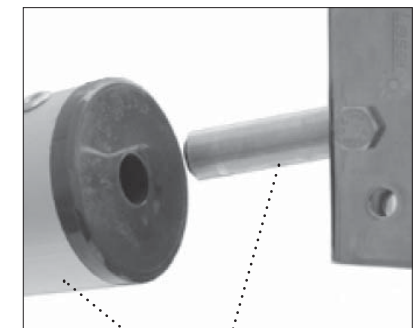
figure 30b | boom, gooseneck pin
